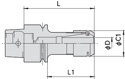
Fig.2 HSKE-CTS
